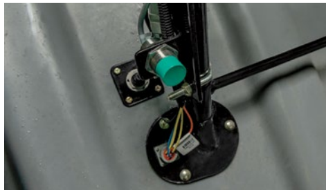
Low level tank sensor.
